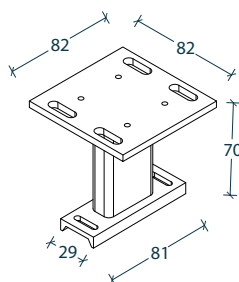
Double Mounting Bracket
