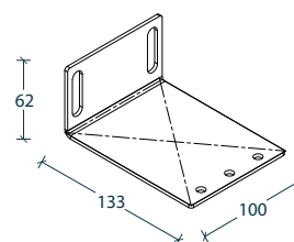
L Mounting Bracket
