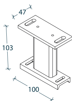
Single Mounting Bracket
