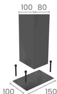
Pergola Foot Profile
