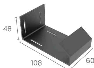
Wall Assemble Part
