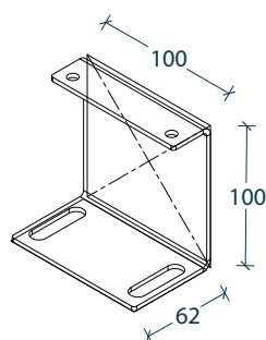
C Mounting Bracket
